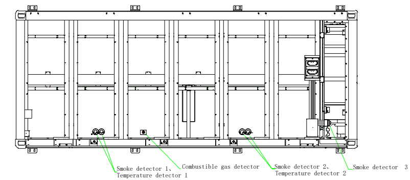
Top view( Remove roof panel)
